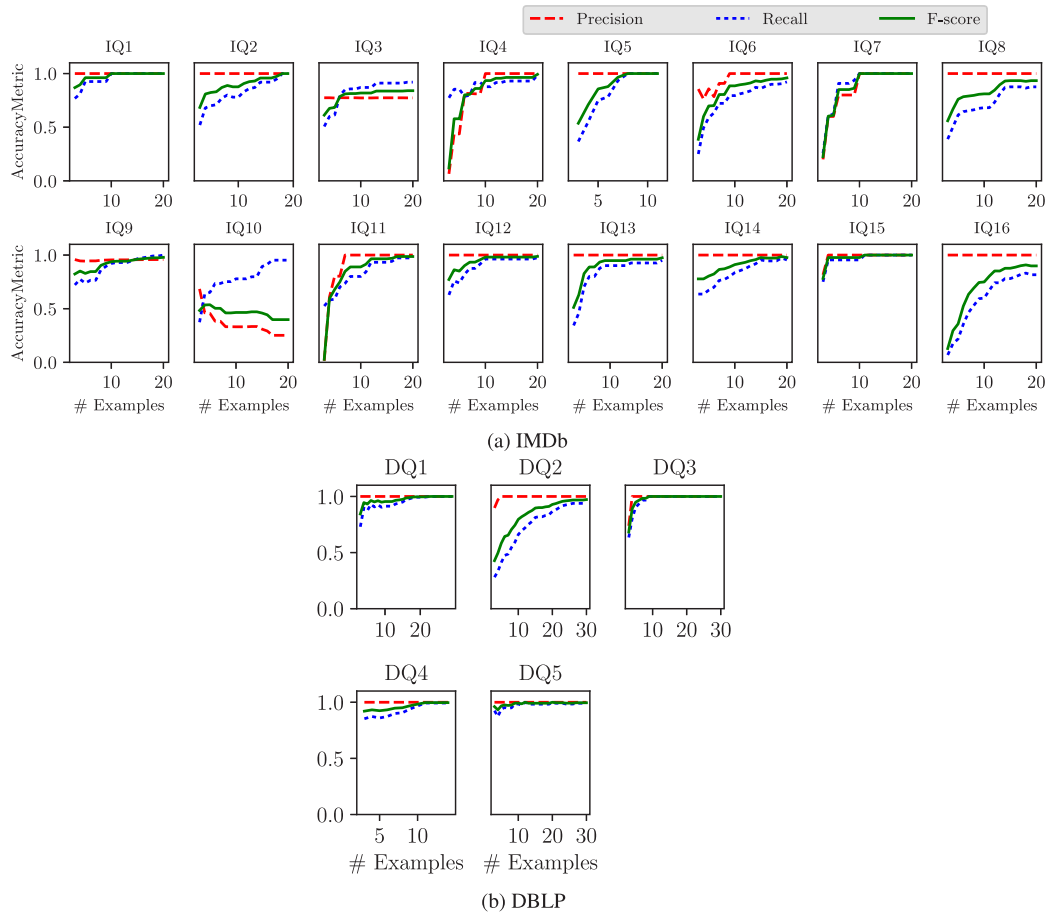
Fig. 10. SQuID achieves high accuracy with few examples (typically \sim 5 ) in most benchmark queries.
