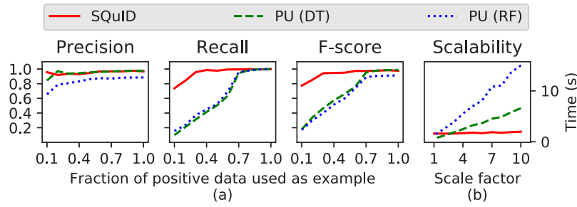
Fig. 16. (a) PU-learning needs a large fraction ( >70\% ) of the query results (positive data) as examples to achieve accuracy comparable to SQUID. (b) The total required time for training and prediction in PU-learning increases linearly with the data size. In contrast, abduction time for SQUID increases logarithmically.
